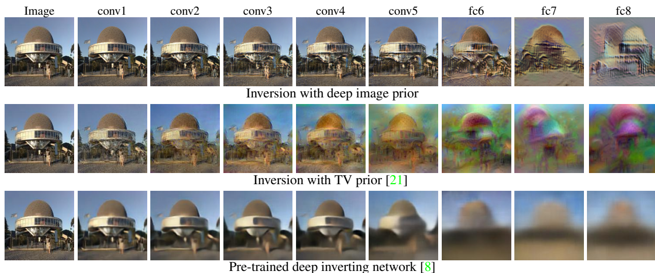
Figure 9: AlexNet inversion. Given the image on the left, we show the natural pre-image obtained by inverting different layers of AlexNet (trained for classification on ImageNet ISLVR) using three different regularizers: the Deep Image prior, the TV norm prior of [21], and the network trained to invert representations on a hold-out set [8]. The reconstructions obtained with the deep image prior are in many ways at least as natural as [8], yet they are not biased by the learning process.
